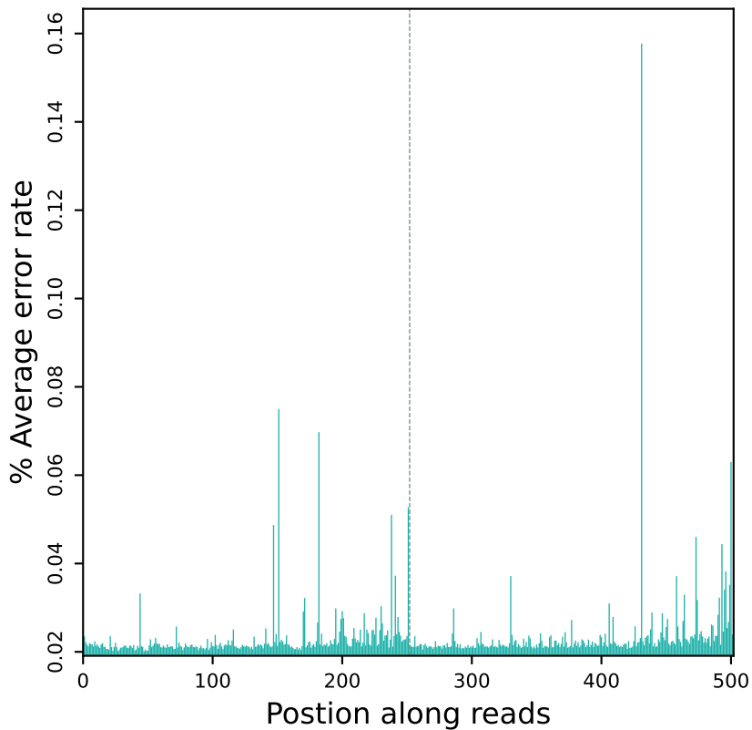
Error rate distribution along reads (R10807)
